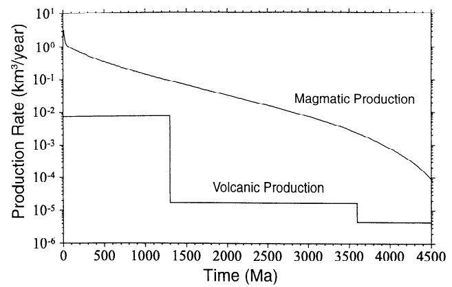
Figure 6. Plot showing the modeled lunar magmatic production rate as a function of time. The estimated basaltic production rate is taken from Head and Wilson [1992].
