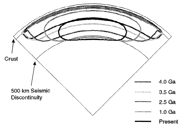
Plate 1. Plot showing the maximum spatial extent of melting beneath the Procellarum KREEP Terrane at times of 4, 3.5, 2.5, 1 and 0 billion years before the present. This cross section spans \pm 45^\circ of latitude, whereas the PKT covers \pm 40^\circ .
