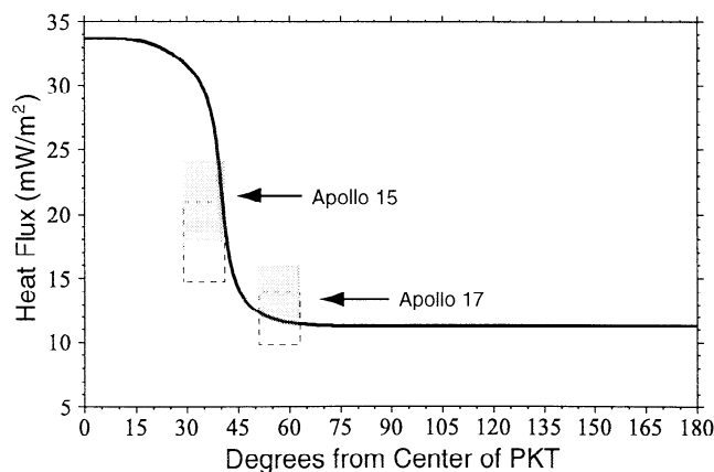
Figure 5. Plot showing the modeled present-day surface heat flux as a function of distance from the center of the Procellarum KREEP Terrane. Also shown are the Apollo heat flow measurements (gray boxes) at their approximate distance from the center of the PKT. The estimated heat flux at these sites after correction for a possible enhancement due to their location at a mare/highlands boundary [Warren and Rasmussen, 1987] is given by the dotted boxes.
