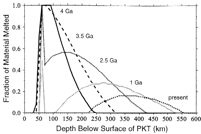
Figure 4. Plot showing the fraction of material melted beneath the center of the PKT at times of 4, 3.5, 2.5, 1, and 0 billion years before the present.
