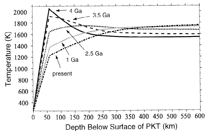
Figure 3. Plot showing the temperature beneath the center of the PKT at times of 4, 3.5, 2.5, 1, and 0 billion years before the present.
