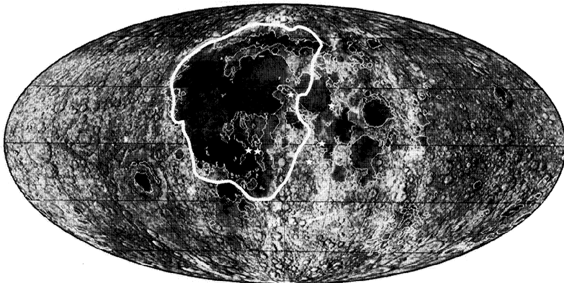
Figure 1. Areal extent of the Procellarum KREEP Terrane (thick line) overlaid on a lunar shaded relief map. The confines of the PKT are here defined by the 3-ppm thorium contour (using the empirical calibration of Gillis et al. [1999]). Thorium concentrations inside of this province average about 5 ppm but are locally as high as 9 ppm. The surrounding highlands, in contrast, are typically lower than 1 ppm. Stars represent the locations of the Apollo landing sites, and the thin lines represent the mare/highland contacts as mapped by Wilhelms [1987]. The surface area of the Procellarum KREEP terrane is about 16% of the Moon's total surface area.
