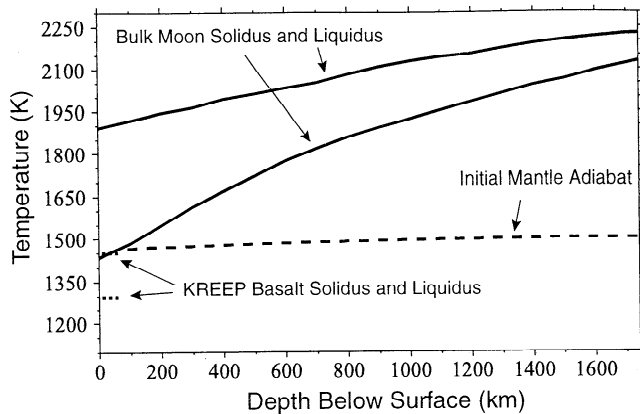
Figure 2. Plot of the bulk Moon liquidus and solidus of Ringwood [1976] and the KREEP basalt liquidus and solidus of Rutherford et al. [1996]. Also shown is the initial adiabatic temperature profile of the mantle.
