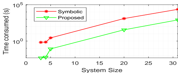
Fig. 9. Computational Time
