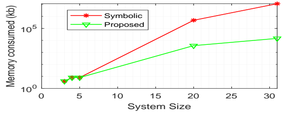
Fig. 10. Computational Memory
