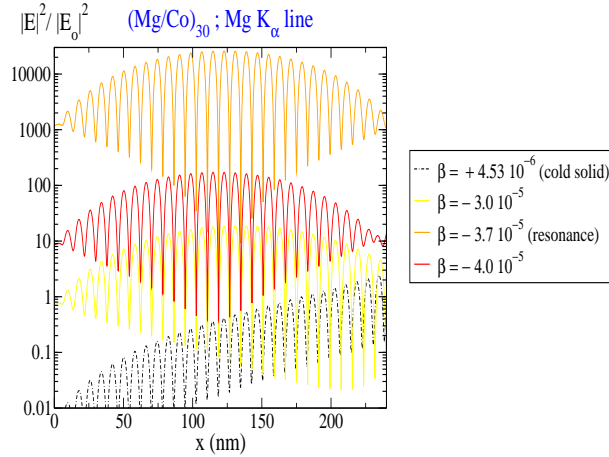
FIG. 8: (Color online) Square of the electric field at the Mg K_\alpha energy (1253.6 eV) inside the (\text{Mg}/\text{Co})_{30} stack ( e_1 = 5.45 nm, e_2 = 2.55 nm), for different imposed values of the imaginary part of the refractive index in the Mg layers. Here, \tilde{n}_{Mg} = 1 - 1.52149 \cdot 10^{-4} - i \beta while \tilde{n}_{Co} = 1 - 9.99187 \cdot 10^{-4} - i 3.97076 \cdot 10^{-4} . Results are normalized to an incident intensity |E_0|^2 .
