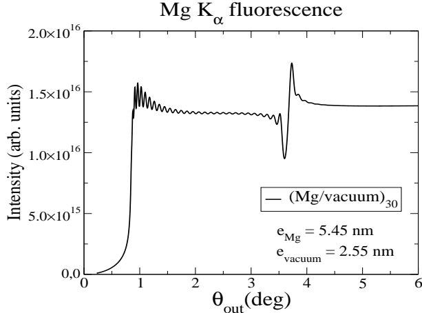
FIG. 7: (Color online) Calculated angular scan for the Mg K_\alpha line emitted by a stack (\text{Mg}/\text{vacuum})_{30} . A uniform excitation (K-shell hole production) has been supposed through the whole sample.
