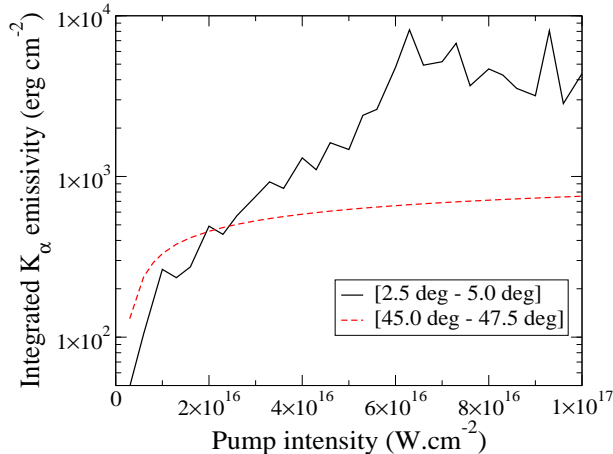
FIG. 12: (Color online) Time integration (over the pulse) and angular integration of the outgoing Mg K_\alpha emissivity as a function of the (XFEL) pump intensity for a 10 fs duration Gaussian pulse of 1332 eV photons. The sample is a (\text{Mg}/\text{Co})_{30} stack with e_1 = 5.45 nm and e_2 = 2.55 nm. - Solid line : integration on the interval [2.5^\circ - 5^\circ] (around the first Kossel pattern) - Dashed line : integration on the interval [45^\circ - 47.5^\circ] (out of the Kossel directions).
