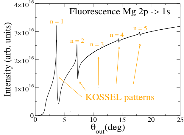
FIG. 4: (Color online) Calculated angular scan for the Mg K_\alpha line emitted by a stack (\text{Mg}/\text{Co})_{30} ( e_1 = 5.45 nm and e_2 = 2.55 nm) irradiated by x-rays above the Mg K-edge. Kossel patterns are labelled by their Bragg order n .
