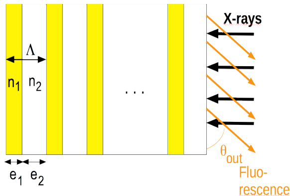
FIG. 2: (Color online) Sketch of a stack of bilayers (of two different elements) excited by x-rays above an absorption edge (K, L or M) in one of the two elements. This results in a K_{\alpha,\beta} , L_{\alpha,\beta,\gamma,\dots} or M_{\alpha} fluorescence emission which can be observed as a function of a glancing angle \theta_{out} . Thicknesses of a bilayer are e_1 and e_2 , respectively while refractive indices are n_1 and n_2 , respectively. The period is \Lambda = e_1 + e_2 .
