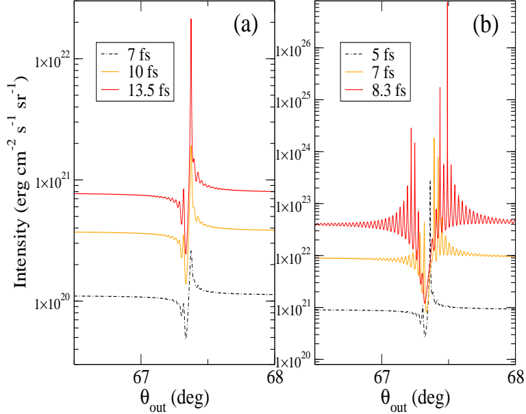
FIG. 16: (Color online) Angular scan of the Si K_\alpha emission, at different times during the transverse irradiation (along the y axis, cf Fig. 1) of the stack (\text{Si}/\text{vacuum})_{5000} ( e_1 = 0.1309 nm, e_2 = 0.2541 nm) by Gaussian pulses, 10 fs duration (FWHM), of 1900 eV photons. (a) 10^{16} W/cm ^2 . (b) 10^{17} W/cm ^2 . Thickness (along the y axis) is less than one \mu\text{m} .
