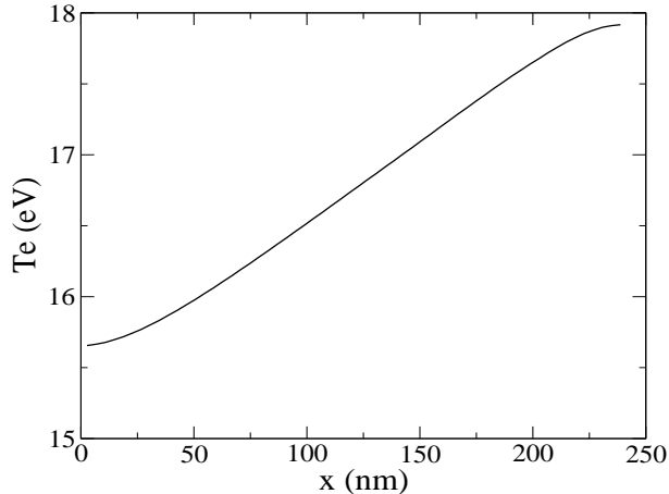
FIG. 11: (Color online) Spatial profile of electronic temperature at the end of the x-ray pulse , in a (\text{Mg}/\text{Co})_{30} stack of period \Lambda = 8 nm, irradiated at normal incidence by a Gaussian XFEL pulse at 10^{16} W/cm 2 , of 1332 eV photons, and of 10 fs duration (FWHM). The x-ray pulse comes from the right.
