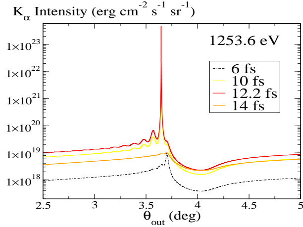
FIG. 10: (Color online) Snapshots of the outgoing Mg K_\alpha emission from a (\text{Mg}/\text{Co})_{30} stack in real pumping conditions (1332 eV photons, 10^{16} W/cm ^2 , FWHM 10 fs, normal incidence). Indicated instants correspond to the time elapsed from the moment the pulse enters the multilayer structure (the peak of the pulse being at 12.8 fs).
