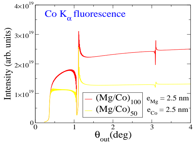
FIG. 5: (Color online) Calculated angular scan for the Co K_\alpha line emitted by two stacks (\text{Mg}/\text{Co})_{50} and (\text{Mg}/\text{Co})_{100} irradiated by x-rays above the Co K-edge.
