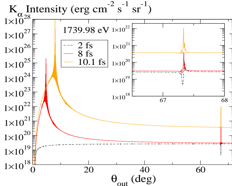
FIG. 15: (Color online) Angular scan of the Si K_\alpha emission, at different times during the irradiation of the stack (Si/vacuum) 10000 ( e_1 = 0.1309 nm, e_2 = 0.2541 nm) by a 10^{17} W/cm 2 Gaussian pulse, 10 fs duration (FWHM), of 1900 eV photons. The inset is a zoom on the Kossel diffraction region around 67 deg.
