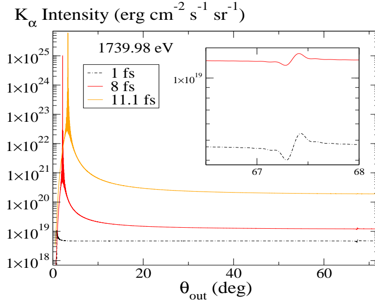
FIG. 14: (Color online) Angular scan of the Si K_\alpha emission, at different times during the irradiation of the stack (\text{Si}/\text{vacuum})_{1000} ( e_1 = 0.1309 nm, e_2 = 0.2541 nm) by a 10^{17} W/cm 2 pulse, 10 fs long, of 1900 eV photons. The inset is a zoom on the Kossel diffraction region around 67 deg.
