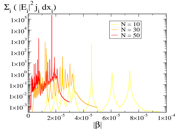
FIG. 9: (Color online) Maximum of the emerging intensity on the Co K_{\alpha 1} found in a glancing angular interval around the first Bragg angle ( \theta_B = 1.025 deg) as a function of the imaginary part of the refractive index of Co. Three stacks (\text{Mg}/\text{Co})_N with e_1 = 2.5 nm, e_2 = 2.5 nm and N = 10, 30, 50 , are considered. Here the pumping is uniform, i.e. arbitrarily j_i = 1 for all cells i .
