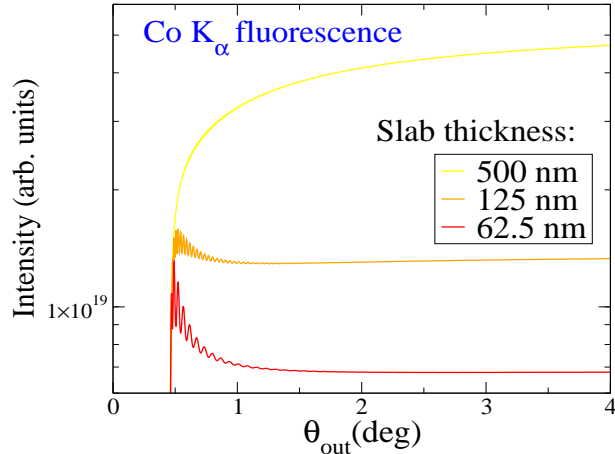
FIG. 6: (Color online) Calculated angular scan around the critical angle for the Co K_\alpha line emitted by slabs of different thicknesses. A preliminary uniform excitation (K-shell hole production) has been supposed over the whole slabs.
