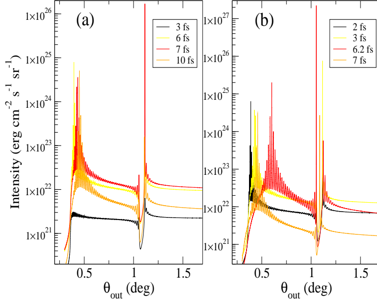
FIG. 13: (Color online) Snapshots of the grazing outgoing Co K_{\alpha 1} emission from a (\text{Mg}/\text{Co})_{50} stack ( e_1 = e_2 = 2.5 nm) in real pumping conditions (7720 eV photons, FWHM 10 fs, normal incidence). (a) 6 \times 10^{18} W/cm ^2 . (b) 3 \times 10^{19} W/cm ^2 .
