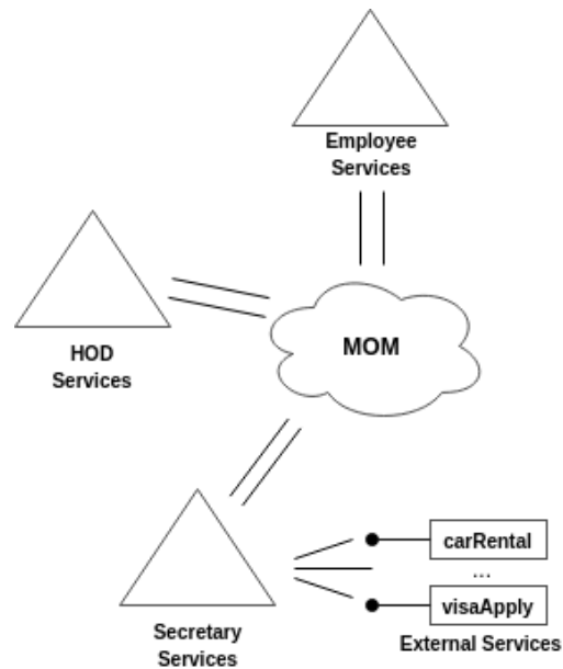
Figure 12. The architectural style of the execution engine is P2P. The employee, the HOD and the Secretary exchange data via MOM-type middleware.
