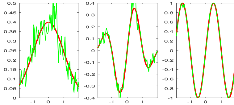
FIG 3. Small bandwidth effect, the ratio of two bad estimators is a good estimator. For bandwidth h = 0.01 and n = 1000 , true (bold) and estimated f (left), b_1 f (middle), and b_1 (right).
