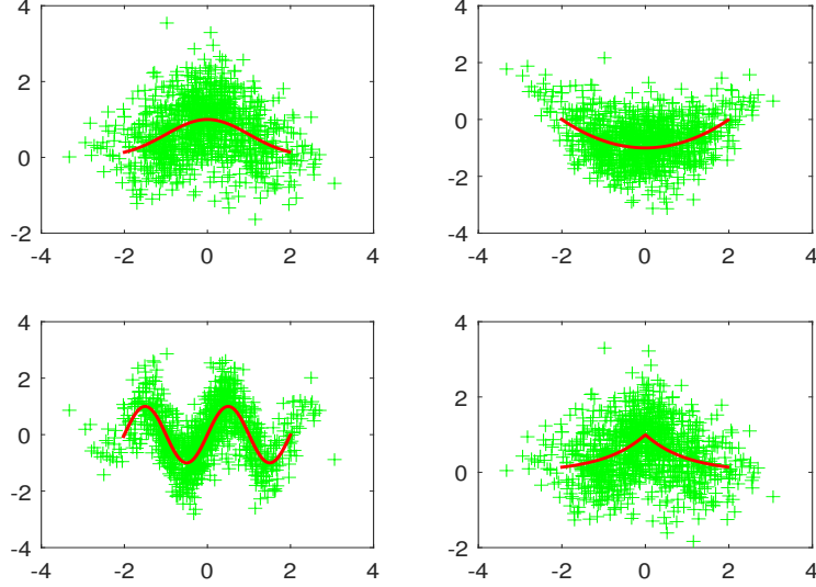
FIG 2. Observations (X_i, Y_i)_{1 \leq i \leq n} for n = 1000 in the four cases of functions b_1 to b_4 , with large noise \sigma = 0.7 , and true regression function in bold red.
