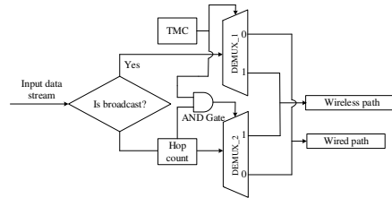
Fig. 5: Dynamic Broadcast Mode Controller circuit.
