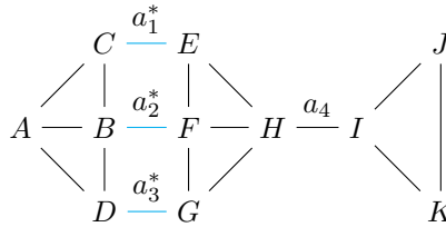
Fig. 4. Graph G_2 .
