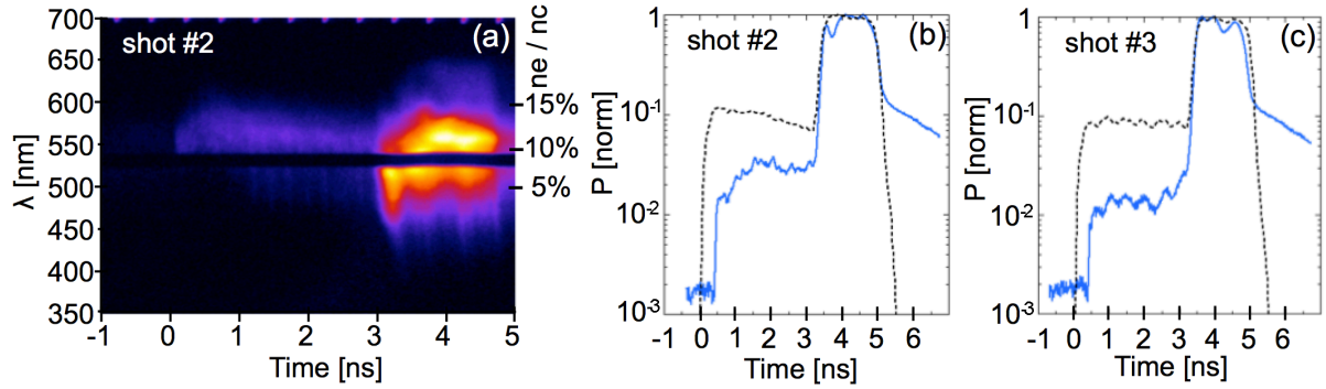
Fig. 3. (a) Time-resolved SRS spectrum for the shot #2 (without SSD). The two graphs show the spectrally integrated SRS signals from the streaked spectra (blue solid line) for shot #2 without SSD (b) and shot #3 with SSD (c). In both graphs, the laser power is shown as black dashed line. All signals are normalized to their respective maximum.
