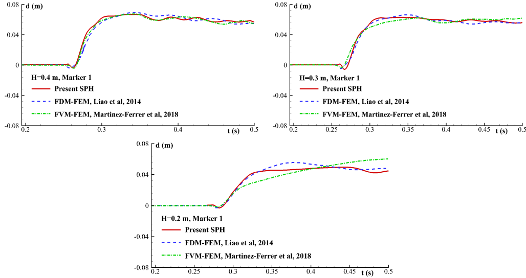
Fig. 18. Time evolutions of the initial horizontal displacements of the marker 1 on the elastic plate in the three dam-breaking flows with the initial water depths as H = 0.4m , 0.3m and 0.2m respectively: the SPH results are compared against the corresponding FDM-FEM results from [27] and the FVM-FEM solution from Martínez-Ferrer et al.[38].
