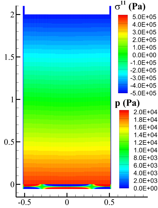
Fig. B.1. The pressure field in the fluid and the field of the stress component \sigma^{11} in the structure at t = 0.1 s.
