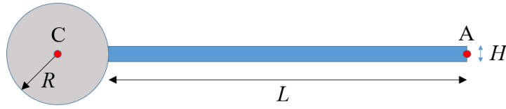
Fig. A.1. Sketch for the benchmark test proposed by Turek and Hron [52] for validating the structure solver.
