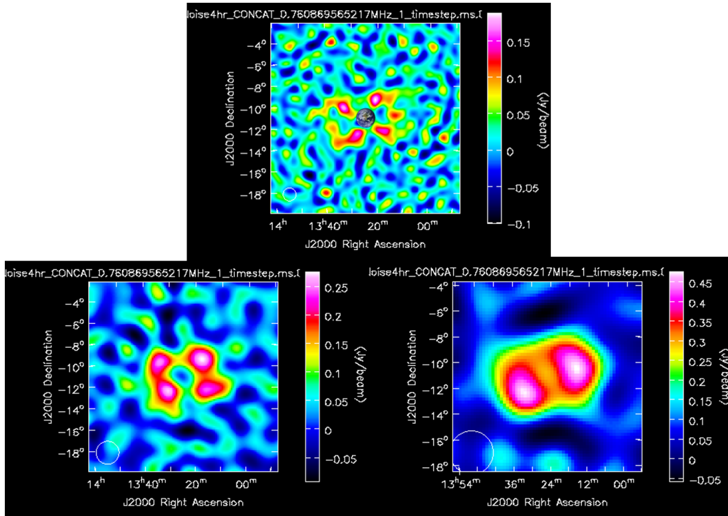
Figure 6: Recovered Dirty Images after 4 hours Integration with Optimal, Amplifier Limited Noise. Top : Noisy response of 20 km array, \sigma = .0318 Jy/beam \implies SNR \approx 3.93 for each lobe. The 1.91^\circ Earth is added in for a scale indicator. Left : Noisy response of 10 km array, \sigma = 0.041 Jy/beam \implies SNR \approx 5.85 for each lobe. Right : Noisy response of 6 km array, \sigma = 0.073 Jy/beam \implies SNR \approx 6.44 per lobe. Images were made with a Briggs weighting scheme with a robustness parameter of -0.5, and are showed here completely un-CLEANed.
