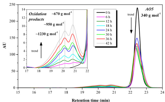
Fig. 7. SEC chromatograms of AO5 acquired at 280 nm at various exposure times at 90 °C under 3.0 MPa oxygen pressure.
