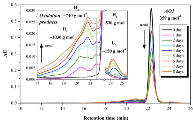
Fig. 3. SEC chromatograms of AO1 acquired at 293 nm at various exposure times at 90 °C under 3.0 MPa oxygen pressure.
