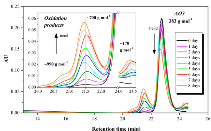
Fig. 5. SEC chromatograms of AO3 acquired at 281 nm at various exposure times at 90 °C under 3.0 MPa oxygen pressure.
