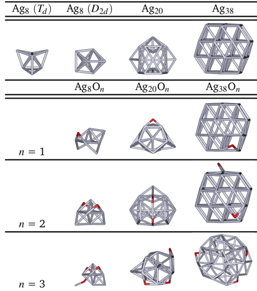
Figure 1: Geometrical structures of pure (Ag 8 with T_d and with D_{2d} symmetry, Ag 20 , and Ag 38 ) and oxidized (Ag m O n , m = 8, 20, 38 , and n = 1, 2, 3 ) silver clusters. The oxygen atoms are represented in red.
