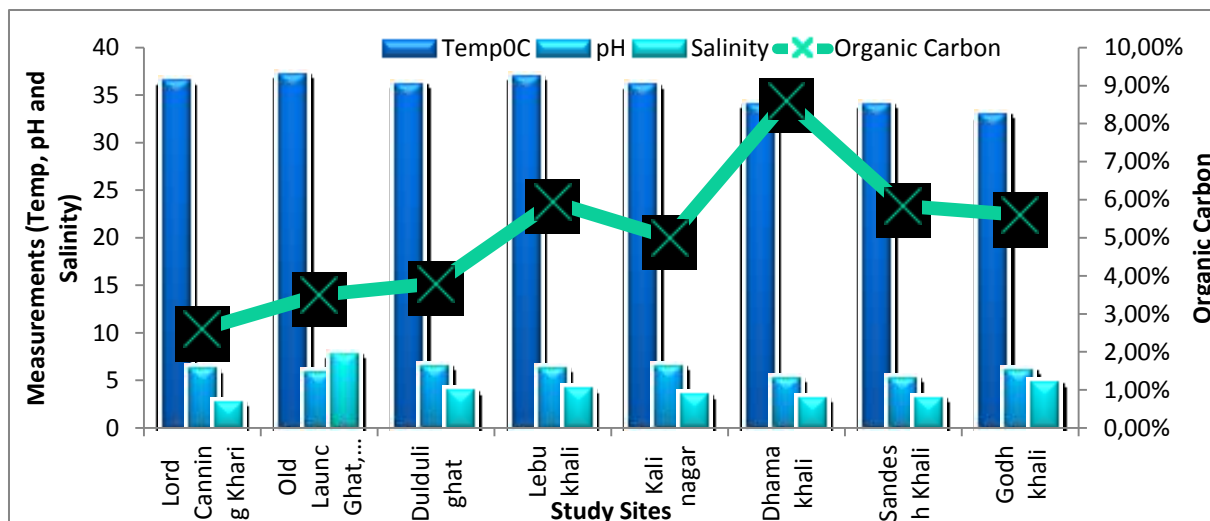
Bar chart showing soil sample test results
