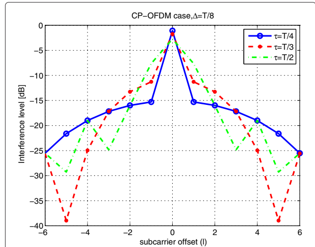
Figure 7 OFDM instantaneous interference tables for \tau = \{T/4, T/3, T/2\} .
