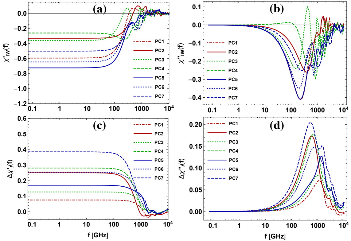
FIG. 6. Dielectric spectra of the pore solutions PC1-PC7: (a) real \chi'_{IW}(f) and (b) imaginary \chi''_{IW}(f) parts of the ion-water dielectric contribution; (c) real \Delta\chi'_I(f) and (d) imaginary \Delta\chi''_I(f) parts of the DC-conductivity dielectric ion contribution.
