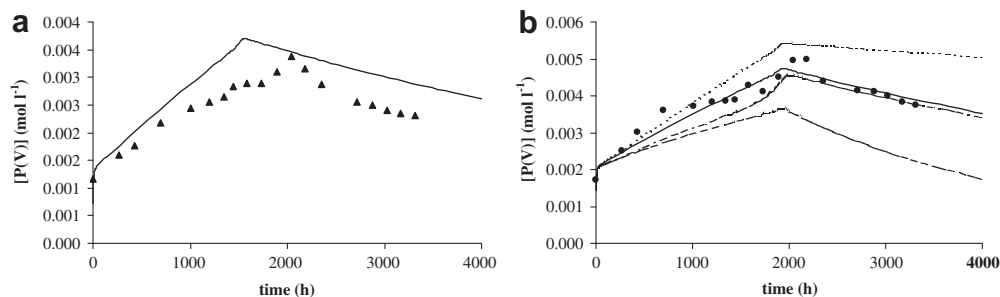
Fig. 10. Phosphate concentration changes with time at 80 °C in air for PE + 0.3% ( \blacktriangle ) and PE + 0.4% Irgafos 168 ( \bullet ) together with kinetic modelling (full lines) using parameters given in Tables 3 and 4. (...) corresponds to a simulation with H_{Dec=0} = 10^{-8} \text{ s}^{-1} , (---) with H_{Dec=0} = 10^{-7} \text{ s}^{-1} , and (- · - ·) with s_{Dec} = 0.003 \text{ mol l}^{-1} and k_{Dec} = 0.02 \text{ l mol}^{-1} \text{ s}^{-1} .
