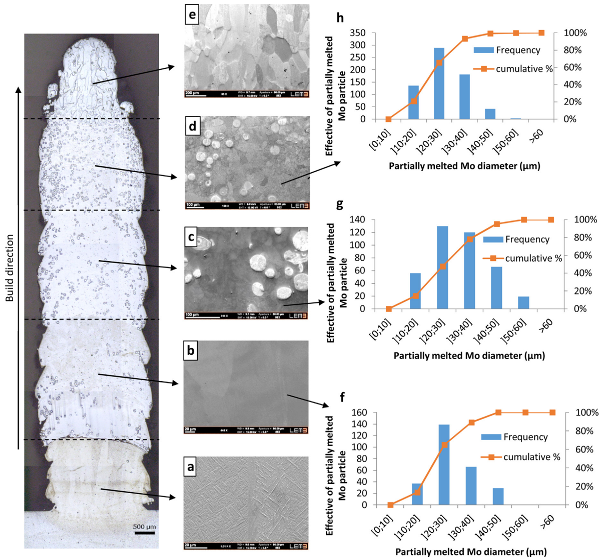
Fig. 9. Evolution of the microstructure of Ti6Al4V-Mo alloys with Mo content (wt.%) (a) 0% Mo, (b) 25% Mo, (c) 50% Mo, (d) 75% Mo, (e) 100% Mo. Partially melted Mo grain size distribution for (wt.%) (f) 25% Mo, (g) 50% Mo, (h) 75% Mo.
