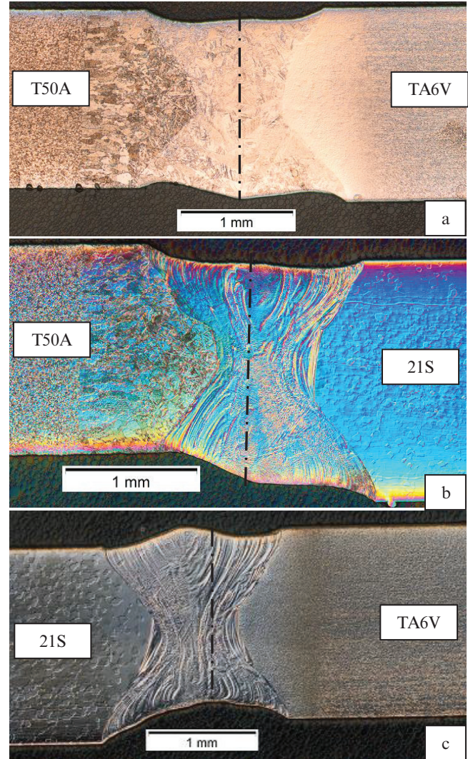
Figure 7: Optical micrographies of: a. T50A/TA6V, b. T50A/21S and c. TA6V/21S ( P=3 kW, v=3 ml/min, \Delta x=0 ). The dotted line represents the initial joint plane
