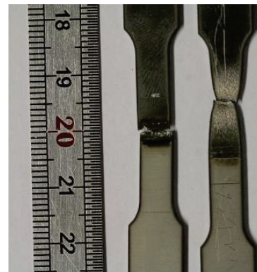
Figure 4: Two tensile test specimen of TA6V/21S after break
