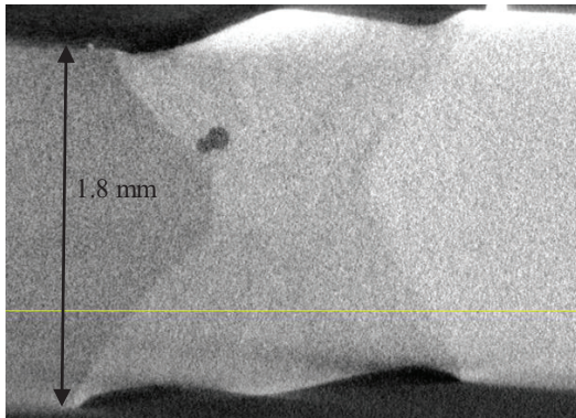
Figure 6: Porosity in the TA6V/21S bead ( P=3 kW, v=3 ml/min and \Delta x=0 mm)
