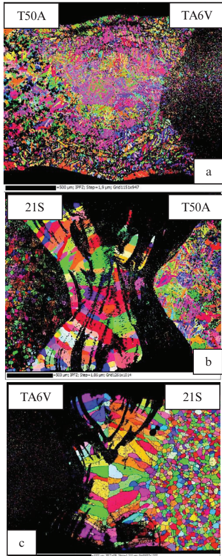
Figure 8 : EBSD Map of: a. T50A/TA6V, b. T50A/21S and c. TA6V/21S ( P=3 kW, v=3 m/min and d=0 mm)
