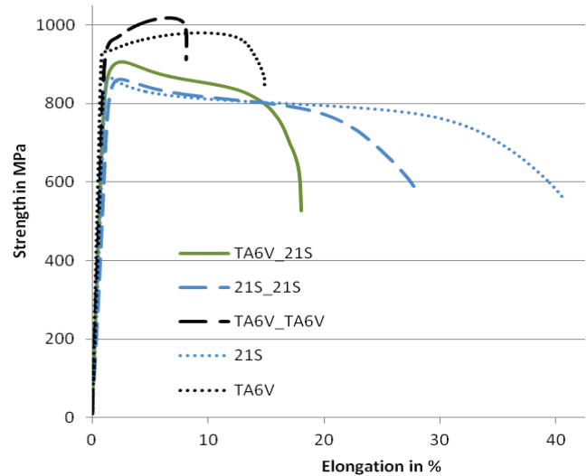
Figure 3: Tensile test of TA6V/21S couple ( P=2.5\text{ kW} , v=2.5\text{ m/min} , \Delta x=0 )
