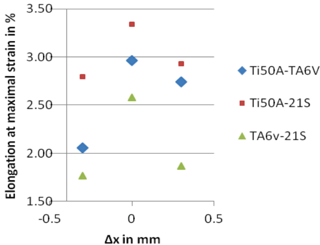
Figure 10: Elongation at maximal strain as function as beam offset from the joint line ( P=2.5 kW and v=2.5 ml/min)
