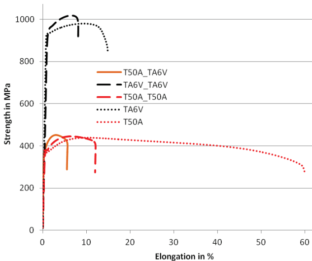
Figure 1: Tensile test of T50A/TA6V couple ( P=2.5\text{ kW} , v=2.5\text{ m/min} , \Delta x=0 )
