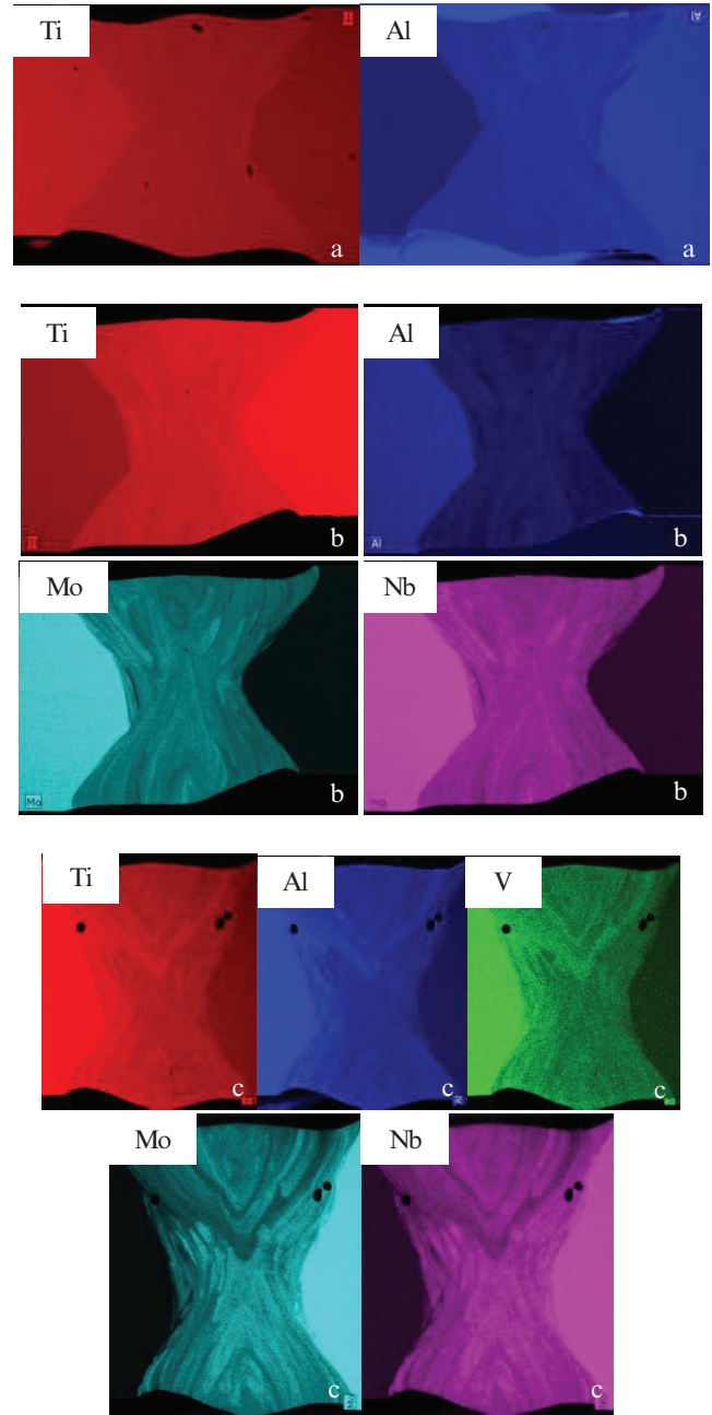
Figure 9: EDX Map of: a. T50A/TA6V, b. 21S/T50A and c. TA6V/21S ( P=3 kW, v=3 m/min and d=0 mm)
