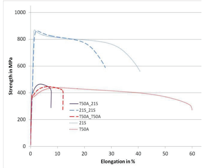
Figure 2: Tensile test of T50A/21S couple ( P=2.5\text{ kW} , v=2.5\text{ m/min} , \Delta x=0 )
