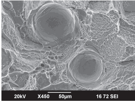
Figure 5: Porosity at the fracture surface of TA6V/21S
