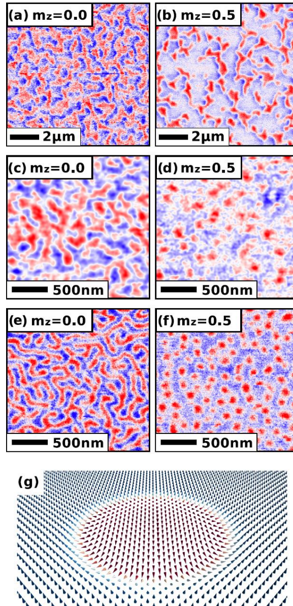
Figure 1: MFM images at 300K for Co/Pt (a)-(b), Ir/Co/Pt (c)-(d), and Ru/Co/Pt (e)-(f) multilayers. For each sample, a series of images was acquired in increasing magnetic fields, to monitor the magnetization reversal from negative ( m_z = -1 ) to positive ( m_z = 1 ) saturation. Images are shown for m_z = 0 and m_z = 0.5 , as estimated from the up/down domain areas. (g) Sketch of a Néel skyrmion, in which cones represent the orientation of the local magnetic moments. The color code highlights the direction of m_z , correspondingly to the MFM images. In images (d) and (f), the skyrmions appear as the red disks.
