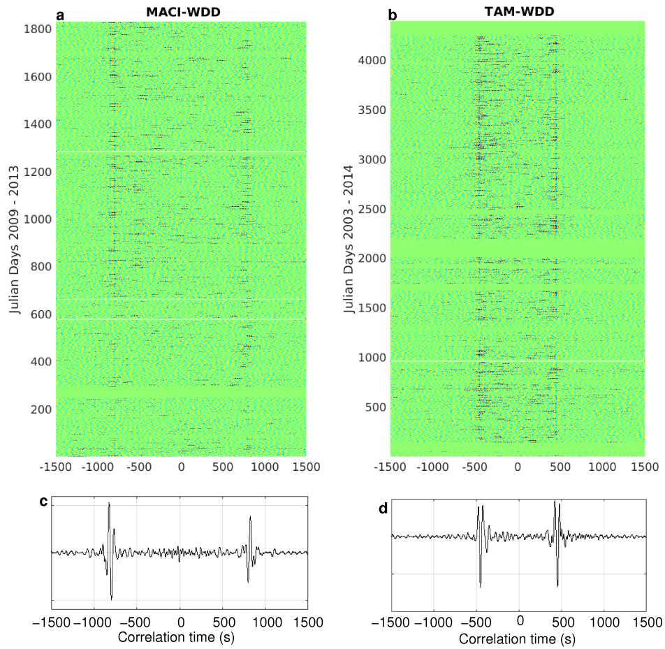
Fig. 5 Cross-correlograms (a, b) and stacks (c, d) filtered between 30 and 100 s for two station pairs. Panels (a) and (c) correspond to the station-pair MACI - WDD (3034 km distance) stacked from 2009 to 2013; pannels (b) and (d) correspond to station pair TAM - WDD (1687 km distance) stacked from 2003 to 2014.
