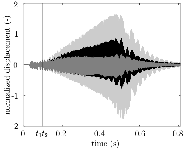
Figure 12. Time evolution of the blade displacement at the leading edge (( \cdots )), mid-chord (( -\cdots- )), and trailing edge (( — )) for the HP compressor test case.
