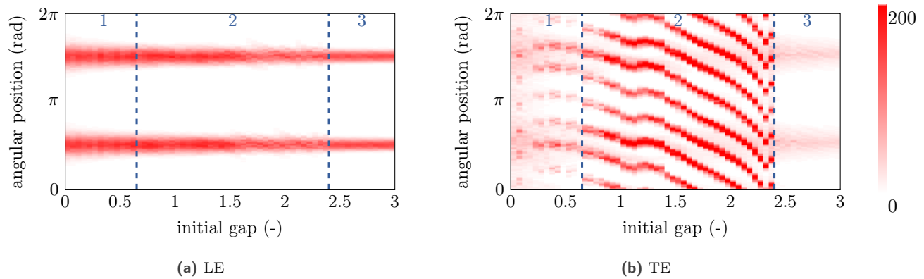
Figure 29. Evolution of the temperature profile with the initial clearance for the LP compressor blade.
