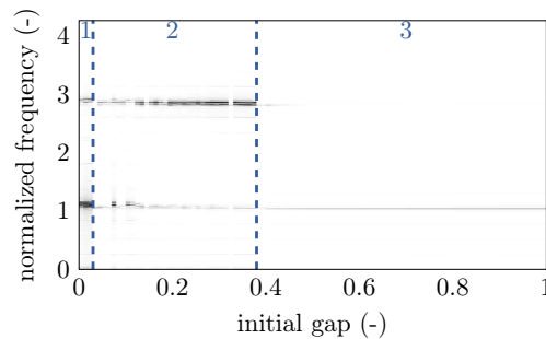
Figure 20. Evolution of the frequency response function of the blade displacement with the initial clearance for the HP compressor blade.
