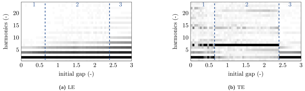
Figure 28. Evolution of the space Fourier transform of the wear profile with the initial clearance for the LP compressor blade.
