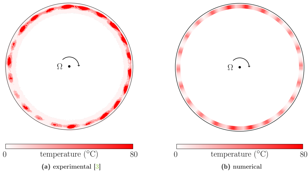
Figure 11. Temperature profile for the HP compressor test case.
