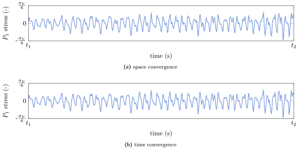
Figure 7. Time evolution of blade stresses (a) with R_s : R_s = 80 (—), R_s = 100 (—), R_s = 200 (—), R_s = 250 (—), and (b) R_t : R_t = 1 (—), R_t = 500 (—), R_t = 1000 (—), R_t = 5000 (—).
