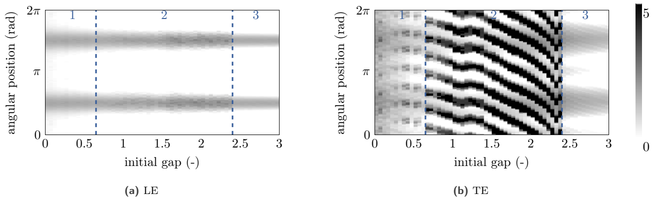
Figure 27. Evolution of the wear profile with the initial clearance for the LP compressor blade.
