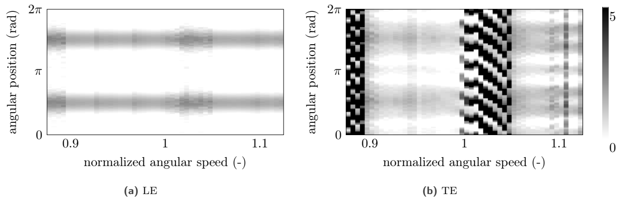
Figure 25. Evolution of the wear profile with the angular speed for the LP compressor blade.
