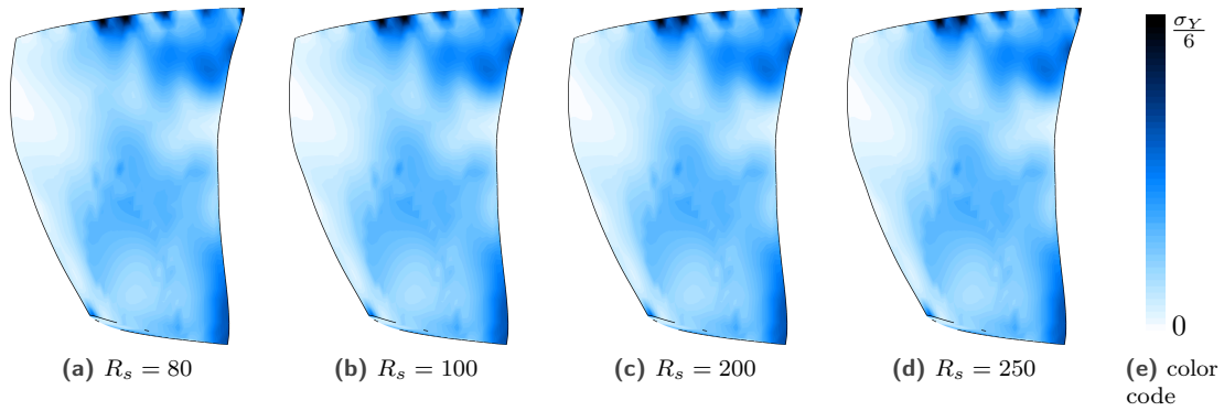
Figure 8. Blade stress fields for different R_s values.
