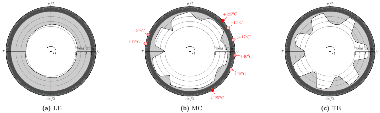
Figure 15. Experimental wear and temperature profiles for the LP compressor test case [2].
