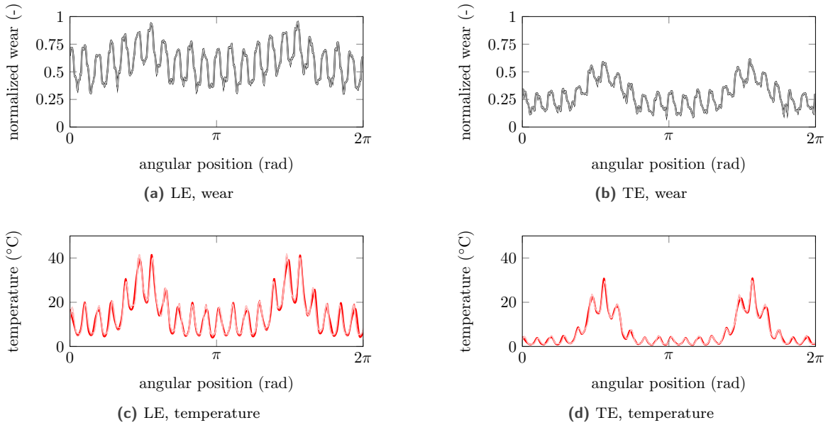
Figure 5. Convergence analysis of the wear and temperature profiles at the end of the simulation at the leading and trailing edge with the number of thermal abratable coating elements n_{ab,th} : n_{ab,th} = 80 or R_s = 250 ((—)/(---)), n_{ab,th} = 100 or R_s = 200 ((—)/(---)), n_{ab,th} = 200 or R_s = 100 ((—)/(---)), n_{ab,th} = 250 or R_s = 80 ((—)/(---)).
