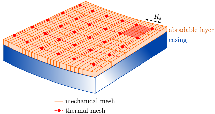
Figure 3. Superimposed mechanical and thermal meshes.
