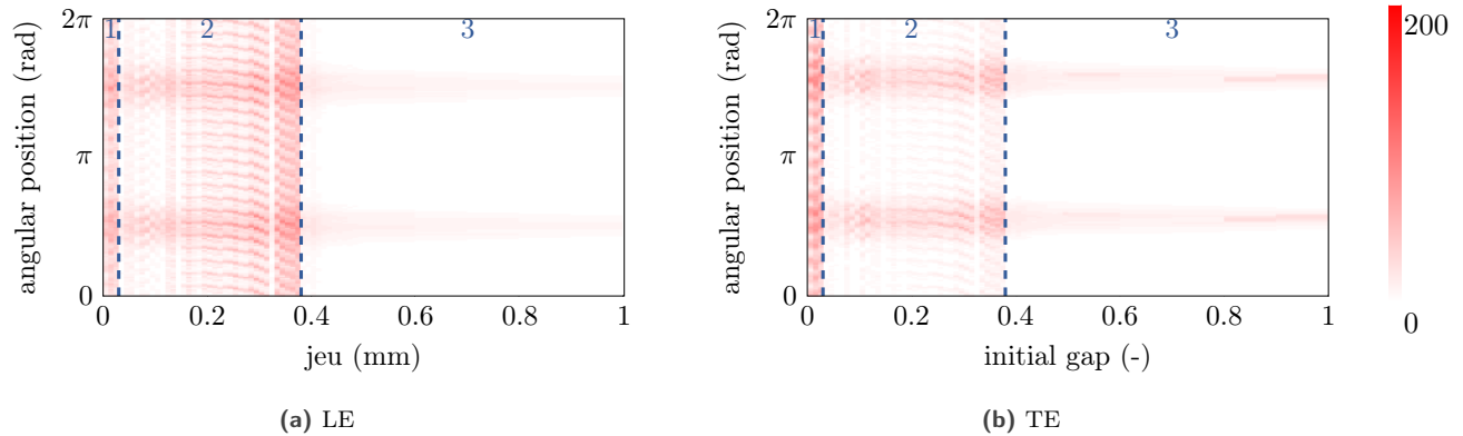
Figure 23. Evolution of the temperature profile with the initial clearance for the HP compressor blade.
