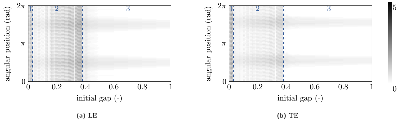
Figure 21. Evolution of the wear profile with the initial clearance for the HP compressor blade.
