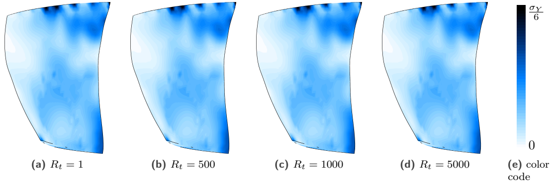
Figure 9. Blade stress fields for different R_t values.
