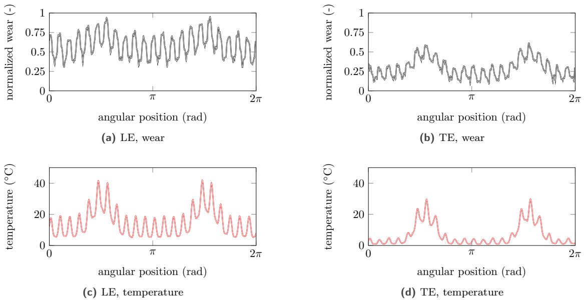
Figure 6. Convergence analysis of the wear and temperature profiles at the end of the simulation at the leading and trailing edge with R_t : R_t = 1 ((—)/(---)), R_t = 500 ((—)/(---)), R_t = 1000 ((—)/(---)), R_t = 5000 ((—)/(---)).
