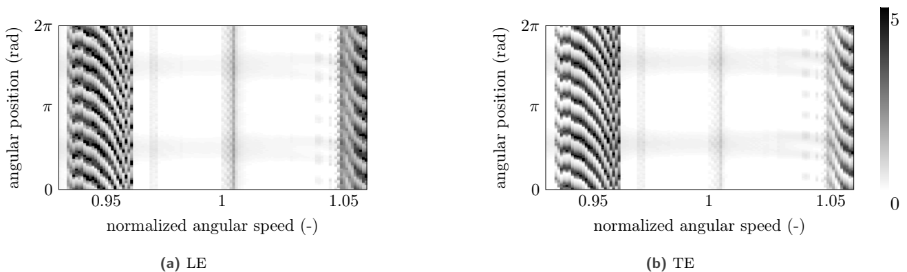
Figure 18. Evolution of the wear profile with the angular speed for the HP compressor blade.
