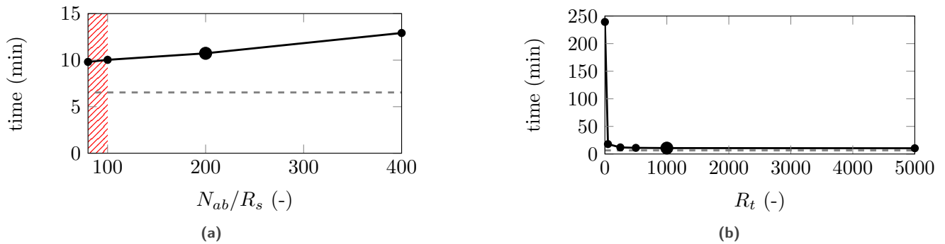
Figure 10. Evolution of the computation time with (a) the number of thermal abradable coating elements, and (b) with R_t .
