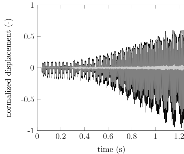
Figure 16. Time evolution of the blade displacement at the leading edge ((—)), mid-chord ((—)), and trailing edge ((—)) for the LP compressor test case.
