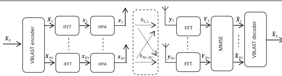
Figure 1 VBLAST MIMO-OFDM system with nonlinear HPA.
