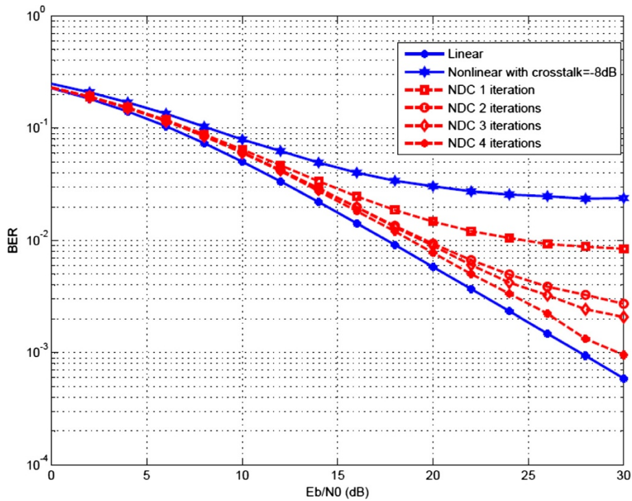
Figure 12 BER versus E_b/N_0 of MIMO-OFDM system with NDC technique for N_c = 64 , N_t = N_r = 2 , IBO = 8 dB, and crosstalk = -8 dB.
