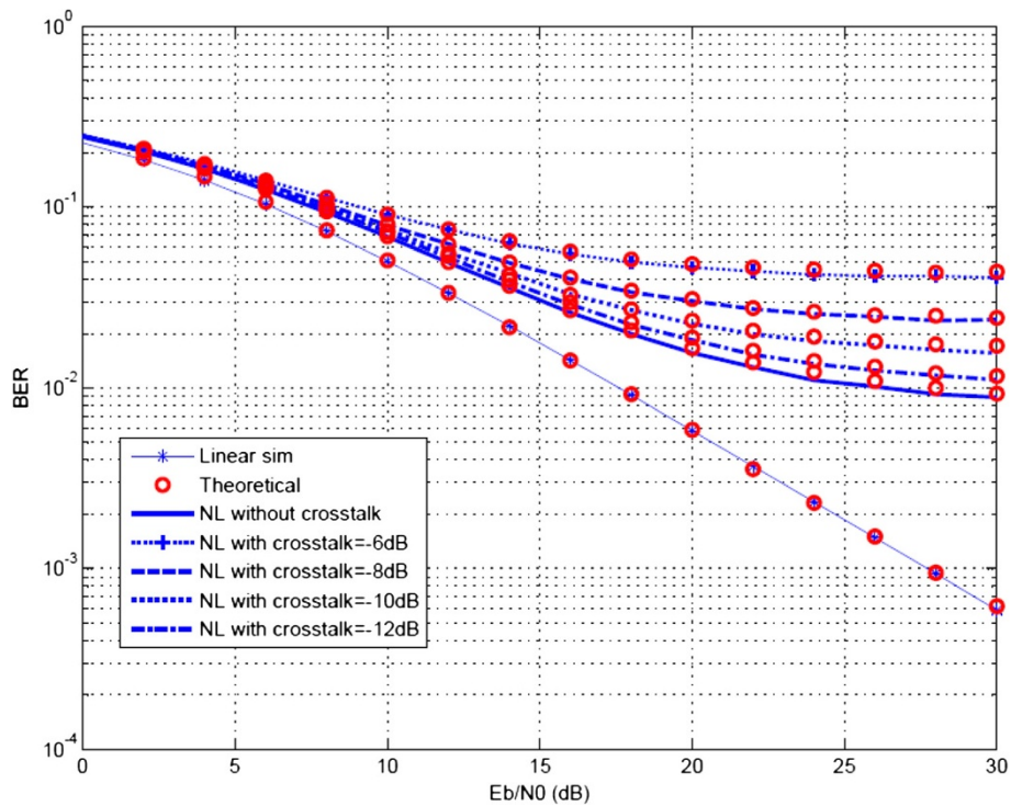
Figure 8 Theoretical and simulation results for BER vs SNR for MIMO-OFDM systems. Polynomial approximation of HPA with 16-QAM, N_c = 64 , N_t = N_r = 2 , IBO = 8 dB, and different values of crosstalk.
