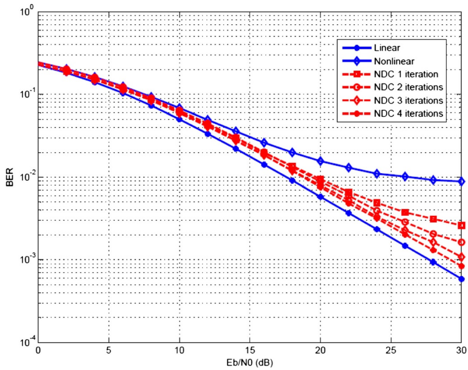
Figure 11 BER versus E_b/N_0 of MIMO-OFDM system with NDC technique for N_c = 64 , N_t = N_r = 2 , and IBO = 8 dB.
