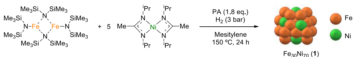
Scheme 1. Synthesis of Fe 30 Ni 70 NPs 1 by co-decomposition of {Fe[N(SiMe 3 ) 2 ] 2 } 2 and Ni[iPrNC(CH 3 )N i Pr] 2 under a H 2 atmosphere.
