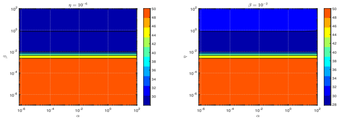
Figure 4. SNR computed for dataset A ( N = 1000 , P = 48 ) using SPOQ regularization with different \alpha , \beta and \eta parameters where p = 0.75 and q = 2 (relative noise: 0.1 %).
