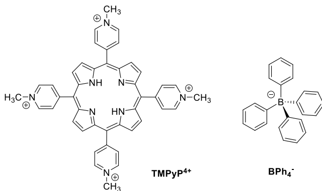
Chart 1. Structures of the TMPP 4+ and BPh 4 - building blocks for the synthesis of porphyrin nanorods.
