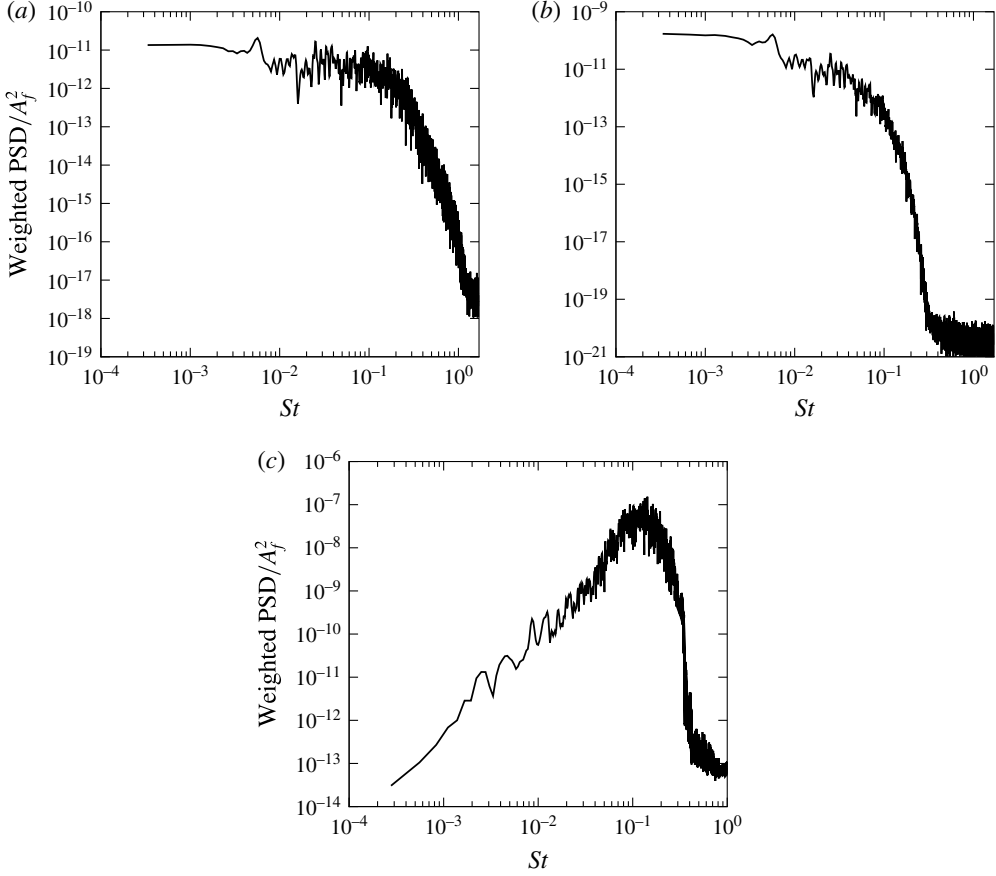
FIGURE 16. M_\infty = 2.15 , \theta = 30.8^\circ and Re_{\delta^*} = 1050 (Case A). Linear regime. Frequency response to internal broadband white noise forcing ( F_2 ) at the (a) separating point; (b) separated shock; (c) downstream position. The WPSDs normalized by the forcing amplitude are represented as a function of the dimensionless frequency ( St ). (a) P_1 – separating point, (b) P_2 – separated shock, (c) P_4 – downstream point.
