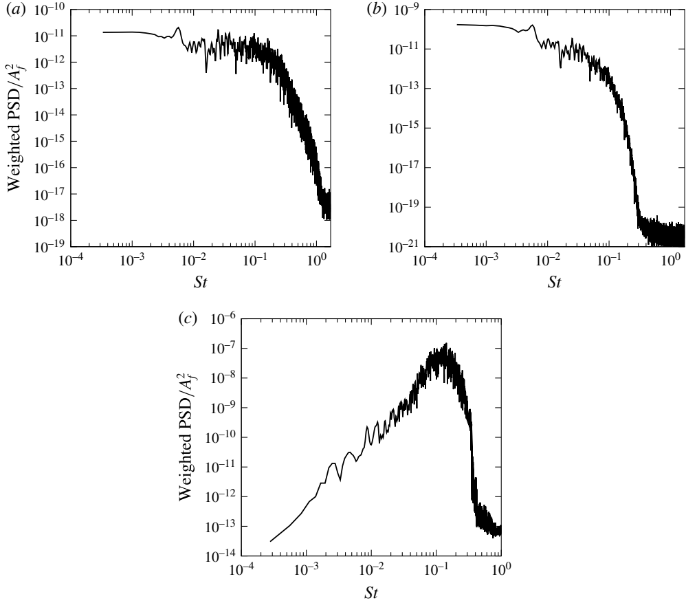
FIGURE 16. M_\infty = 2.15 , \theta = 30.8^\circ and Re_{s^*} = 1050 (Case A). Linear regime. Frequency response to internal broadband white noise forcing ( F_2 ) at the (a) separating point; (b) separated shock; (c) downstream position. The WPSDs normalized by the forcing amplitude are represented as a function of the dimensionless frequency ( St ). (a) P_1 – separating point, (b) P_2 – separated shock, (c) P_4 – downstream point.
