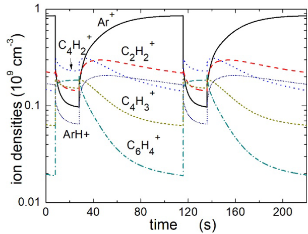
Figure 3. The densities of positive ions as function of time.
