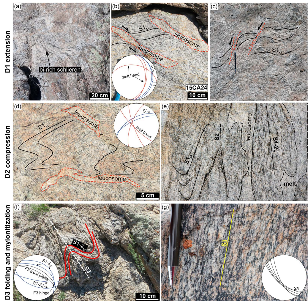
Figure 5. Field photographs illustrating typical structural relationships in the migmatite-magmatite complex. (a) Magmatic fabric ( S1_M ) defined by orientation of restitic Schlieren. (b, c) Migmatitic fabric S1_M is associated with extensional shear bands filled with granitic leucosomes. (d) Transposition of sub-horizontal S1_M foliation by steep melt-bearing S2 foliation and development of axial planar leucosomes of F2 fold. (e) Origin of S1-2_M composite fabric. (f) Character of F3 folding of S1-2_M fabric. (g) Transposition of migmatite-magmatite fabric by mylonitic S3 foliation along the contact with the metamorphosed Habahe Group.
