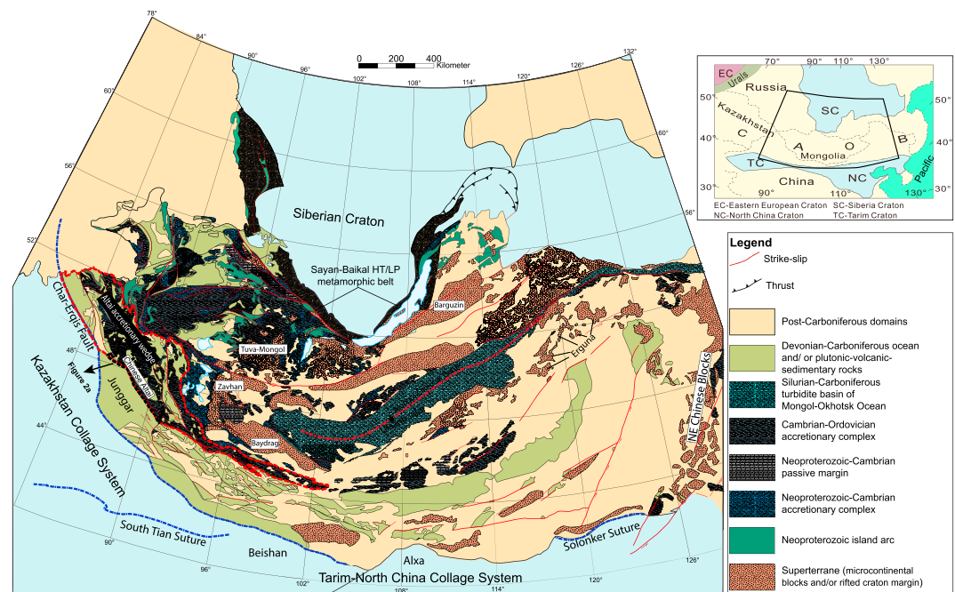
Figure 1. Simplified geological map of the Mongolian Collage System (modified from Jiang et al., 2017). Extent of the Altai accretionary wedge and the location of the Chinese Altai are outlined by dashed lines. Inset shows the position of the Central Asian Orogenic Belt.
