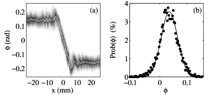
FIG. 3. (a) Average phase distortion \langle \phi(x) \rangle_t in the presence of a vorticity filament. The gray scale corresponds to the probability of observing a given value of \phi around the mean measurement. (b) Probability density function (PDF) of \phi(x = -1 \text{ mm}) ( \bullet ). The solid curve is a Gaussian fit of the experimental PDF. The experimental conditions are 1024 plane emissions at f_0 = 3.5 MHz, L \approx 200 mm, \Omega/2\pi = 5.0 Hz, Q = 3.7 l/min, and D = 80 mm.
