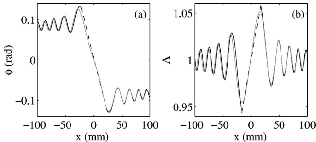
FIG. 14. Comparison between the parabolic equation simulation with \Gamma=470 cm 2 /s and a=0.5 mm (gray lines) and the prediction of Eq. (5.4) with \alpha=0.03 (black solid and dashed lines). (a) Phase and (b) amplitude distortions for a cylindrical emission at f_0=1.5 MHz with L_{\text{em}}=50 mm and L_{\text{rec}}=200 mm. The dashed lines are linear interpolations for the values of x where Eq. (5.4) is not valid.
