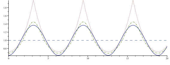
Figure 2. Free surface given by Airy theory (solid line), third order Stokes theory (dash-dot line) and equation (13) (dot line) for the given set of parameters : (a = 1/e, k = 1, c = 1, t = 0, b = 0) .
