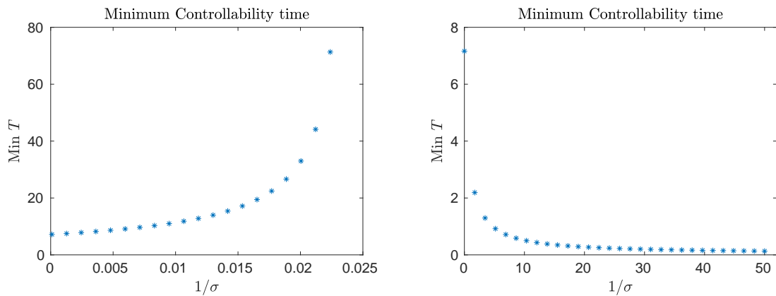
FIGURE 59. Minimal controllability time from 0 to \theta = \frac{1}{3} versus \epsilon = \frac{1}{\sigma} . In the right the minimal controllability time for the Gaussian case N(x) = e^{-\frac{x^2}{\sigma}} , in the right N(x) = e^{\frac{x^2}{\sigma}} .
