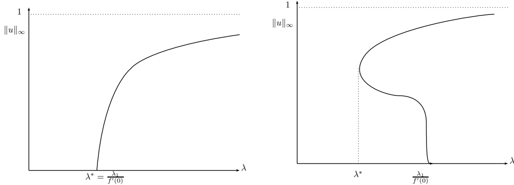
FIGURE 8. Qualitative Bifurcation diagram for the stationary solutions
