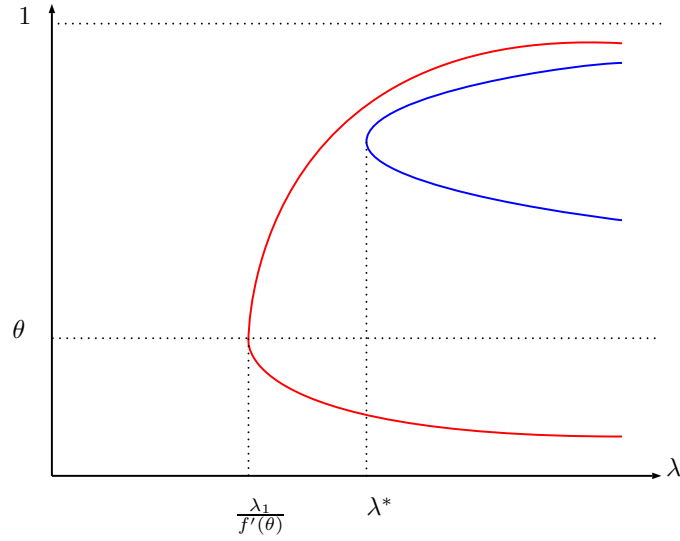
FIGURE 13. Qualitative Bifurcation diagram for the stationary solutions for a bistable nonlinearity which is convex in (0, \theta) and concave in (\theta, 1)
