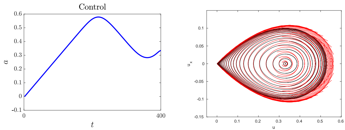
FIGURE 54. (Left) Optimal constrained control associated with Figure 53. (Right) in black steady-states in the phase plane, in red snapshots of the parabolic state in the phase plane
