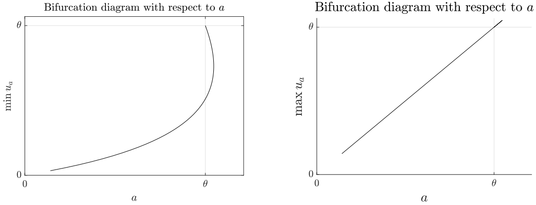
FIGURE 26. In the left, the minimum value of u_a(x) , \min_{x \in [0,L]} u_a(x) is represented against a , for the connected path of steady-states. At the right, the maximum value \max_{x \in [0,L]} u(x) against a
