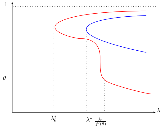
FIGURE 14. Qualitative Bifurcation diagram for a bistable nonlinearity that is convex in (0, p) with p > \theta and concave in (p, \theta) as f(s) = s(1-s)(s-\theta) for \theta < 1/2 .
