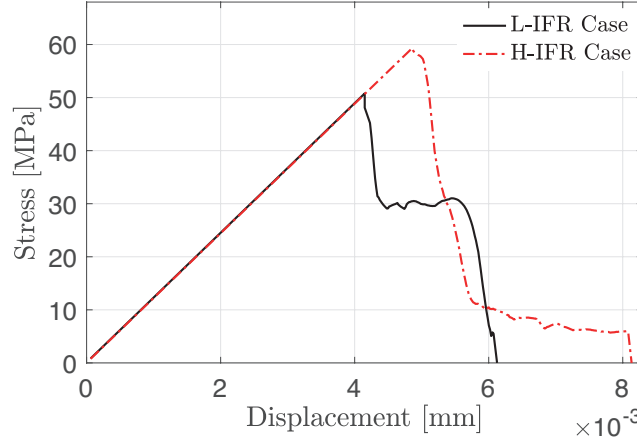
Figure 25: 3D simulation of a structure containing a spherical inclusion, comparison of mechanical response between two cases: low and high interfacial fracture resistance.
