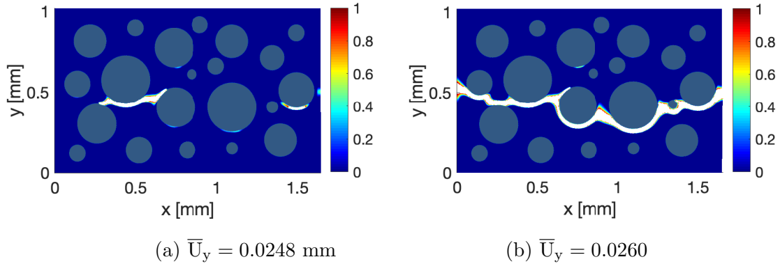
Figure 18: Complex crack paths obtained from the soft interface situation (SI2) with g_c^{si,n} = 6.25 \text{ N/m} , g_c^{si,t} = 5.3 \text{ N/m} . The interfacial cracking is also observed but less than the (SI1) case.
