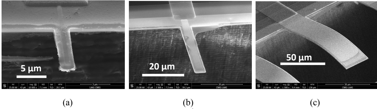
FIG. 2. SEM images of cantilevers with microcontact printed PZT films. (a) Short (10 \mu\text{m} long), (b) medium size (35 \mu\text{m} long) and (c) long (150 \mu\text{m} long) PZT coated cantilevers.
