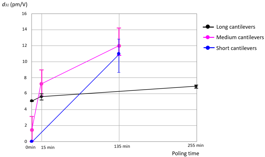
FIG. 12. Evolution of d_{31} (pm/V) as a function of poling time (107 kV/cm at 150°C), for short, medium and long size cantilevers.
