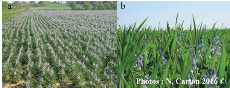
Fig. 1: In Pays de la Loire, market opportunities around Lupin supply triggered the insertion of protein crops on farms. Difficulties encountered in weed infestation for Lupin sole crop (a) can cause the farmer to discontinue it. By contrast, weed management, through Lupin-cereal intercropping for example (b), supports the maintaining of the crop but requires learning through experience and adjustments.
