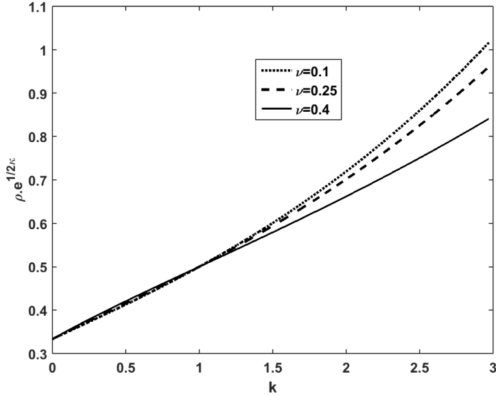
Fig. 8 Variation of \rho e^{1/2\kappa} as a function of the ratio of elastic moduli, for different values of the Poisson's ratio
