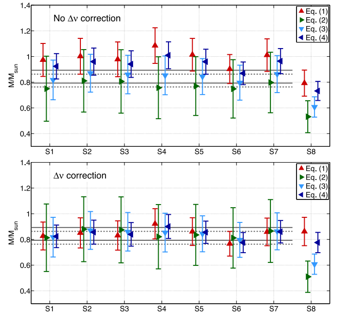
Figure 3. Mass of M4 giants as inferred from equations (1) to (4) with (lower panel) and without (upper panel) applying a model-predicted correction to the \Delta\nu scaling relation. The last star to the right (S8) is an RHB star. The solid and dashed lines denote the 1\sigma mass interval as determined from isochrone fitting and assuming two values for the initial He mass fraction (see Section 3.1.1 for details).
