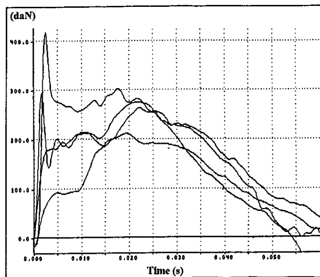
Figure 19 : Superimposing the force curves obtained at the sternum during high speed tests (5.8 m/s) as a function of time.
