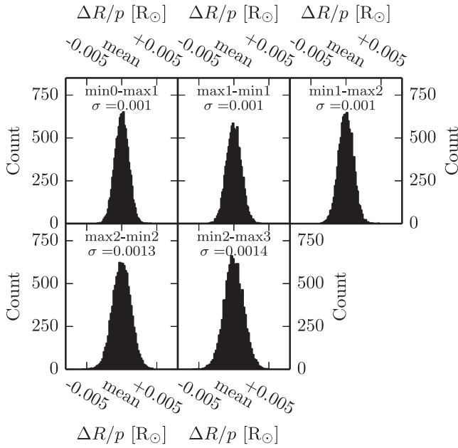
Figure 5. Distributions of \Delta R/p from 10000 Monte Carlo trials, centred on the respective means listed in Table 7. Standard deviations are indicated inside each panel.
