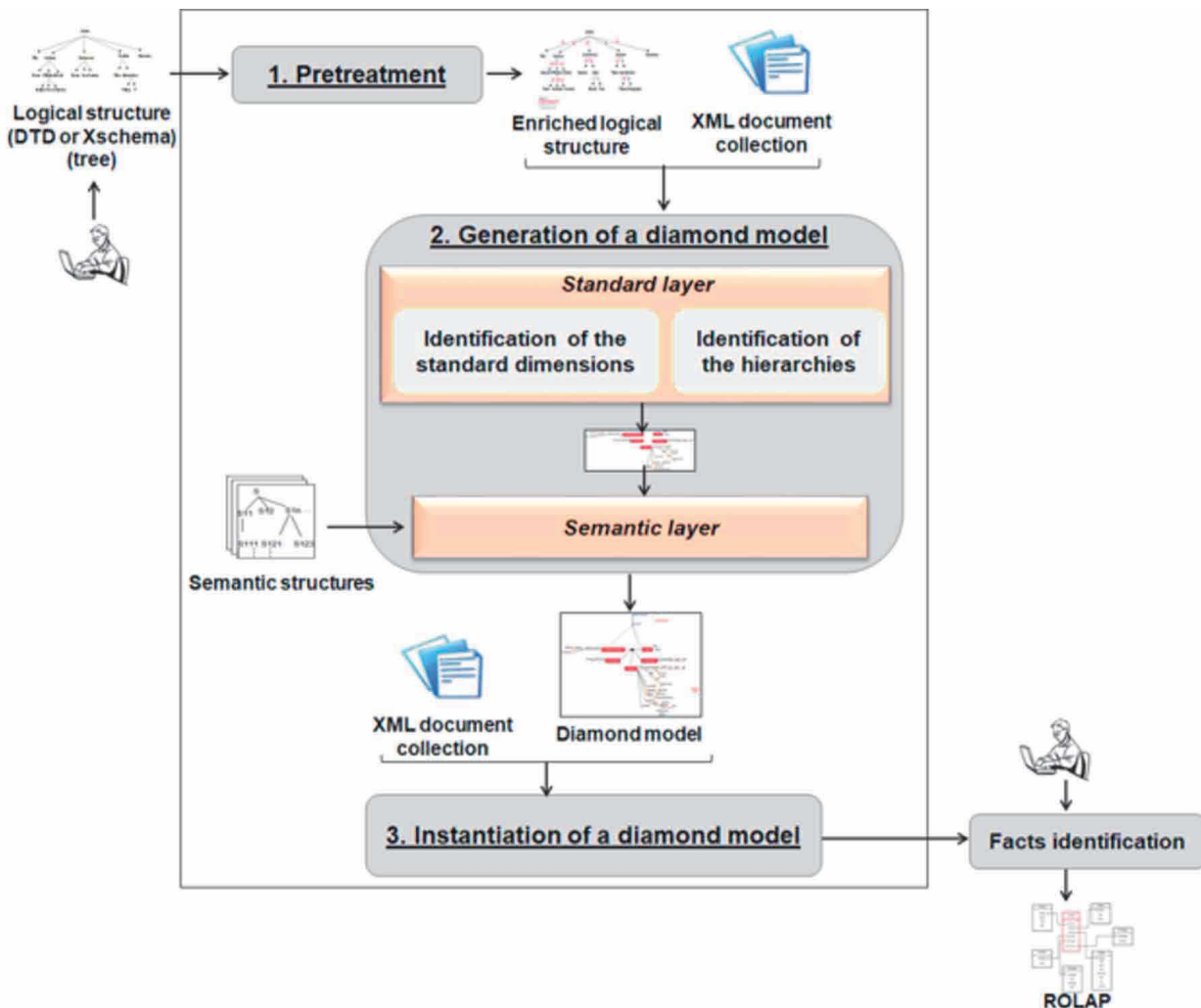
Figure 1. Quasi-automatic approach for the generation of a Diamond multidimensional DOCW model
