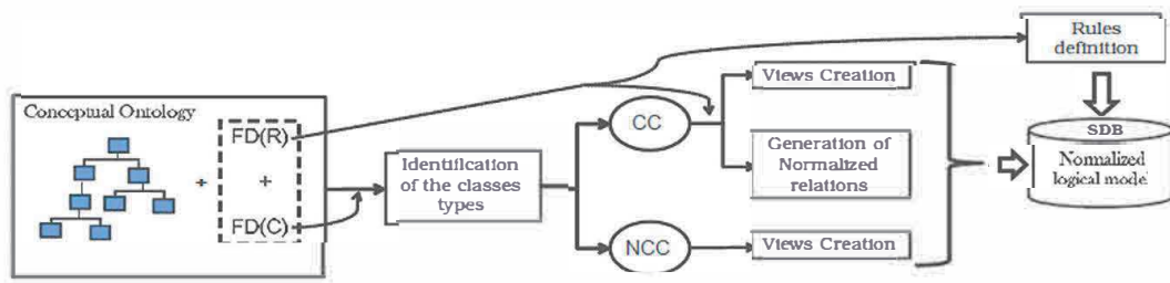
Figure 1: Semantic database design approach.
