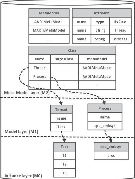
Fig. 3. Data representation in the OntoDB model repository
