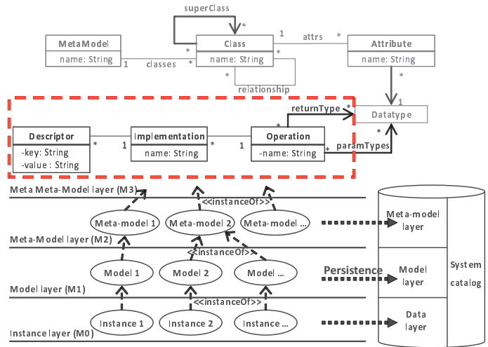
Fig. 2. The architecture of OntoDB/OntoQL
