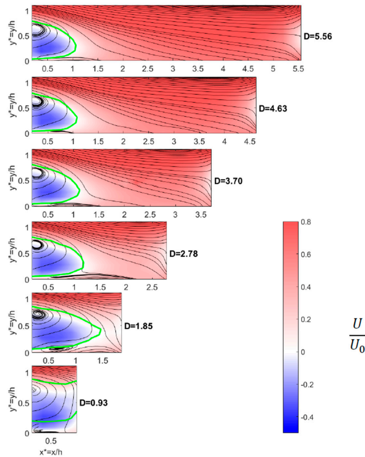
Figure 9. Streamlines and dimensionless streamwise velocity for z^* = 0 for the six inter-vehicle distances D ( \varphi = 35^\circ ). Green lines are isocontours U/U_0 = 0 .
